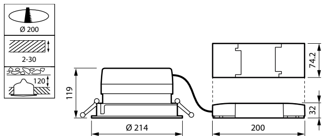
DN571B LED20S/840 PSU-E C WH
