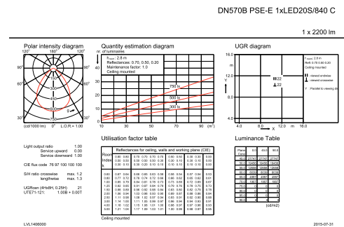
IFGU_DN570B PSE-E 1xLED20S/840 C-General uniform lighting
