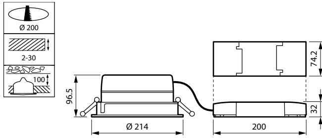
DN570B LED20S/840 DIA-VLC-E C ELP3 WH
