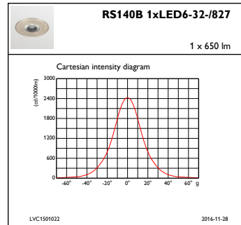
IFCC1_RS140B1xLED6-32-827
