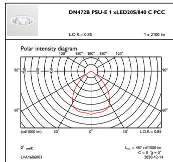
OFPC1_DN472BPSU-E1xLED20S840CPCC
