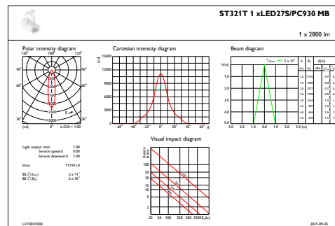
IFAS1_ST321T1xLED27SPC930MB
