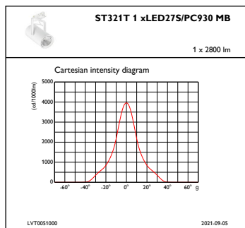
IFCC1_ST321T1xLED27SPC930MB
