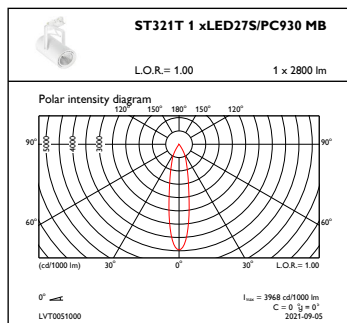
OFPC1_ST321T1xLED27SPC930MB
