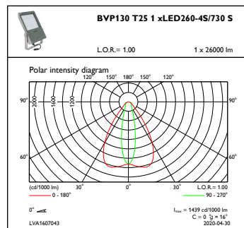
OFPC1_BVP130T251xLED260-4S730S
