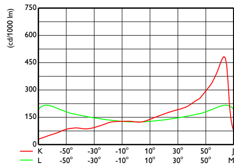
OFCS1_BVP651T251xLED450-4S740DX10
